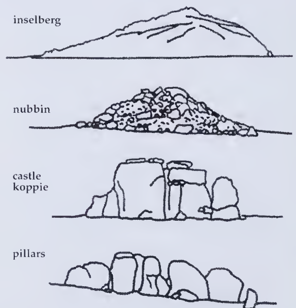
Figure 4. Schematic of major granite landforms (drawn from photographs in Campbell 1997).
